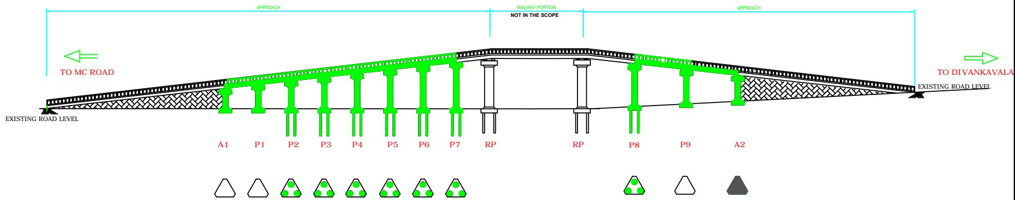
PILE FOUNDATION
